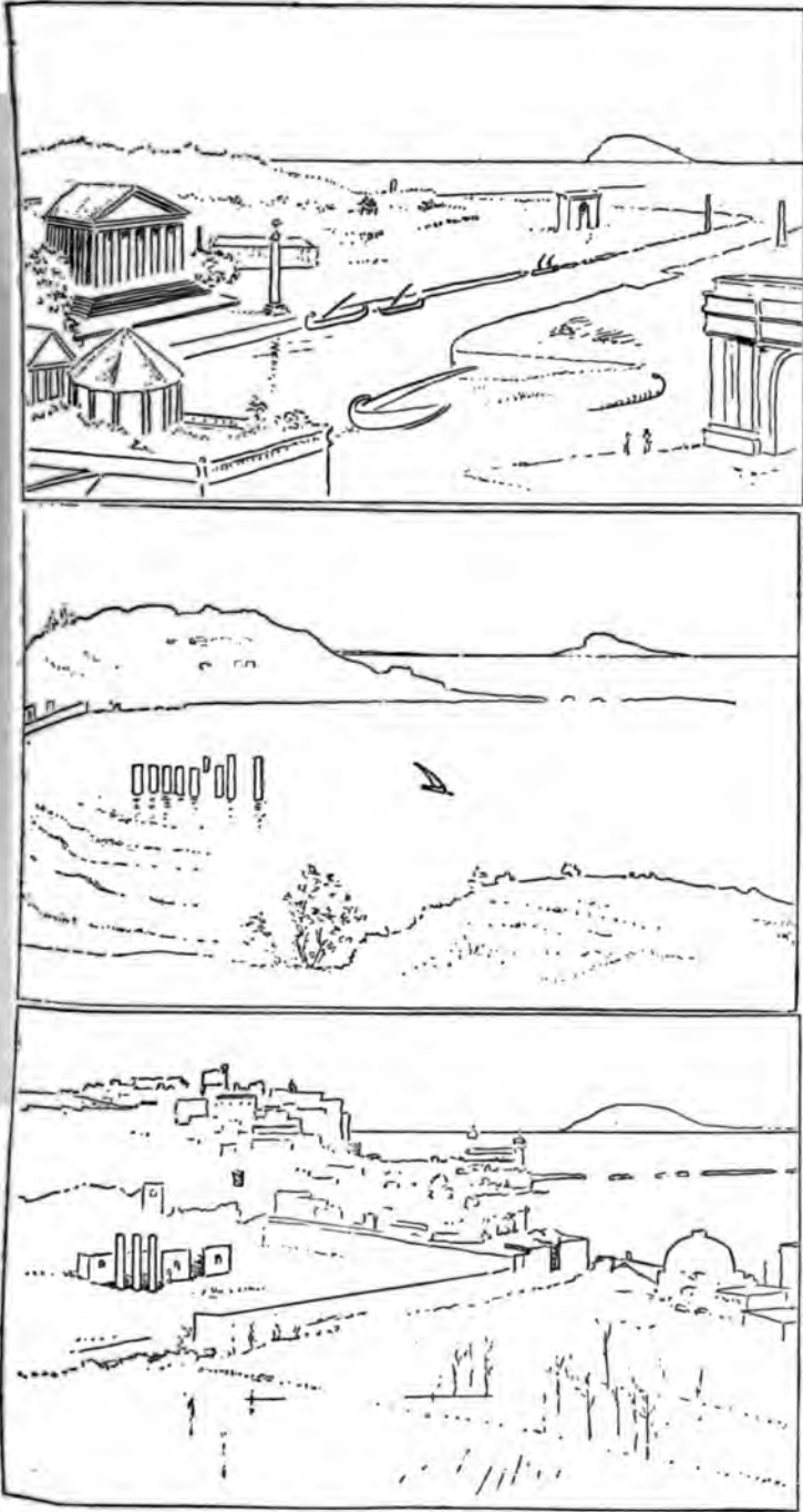
FIG. 286. — Posuoli in the 3rd, 9th, and 20th Centuries.
